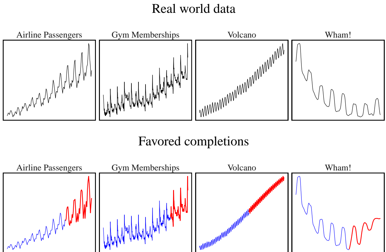
Figure 6. (Top) Real-world data sets used in Experiment 2b. Descriptions and origin of the data were unknown to participants. (Bottom) Participants were shown the region in blue; most frequently selected completions are shown in red.
